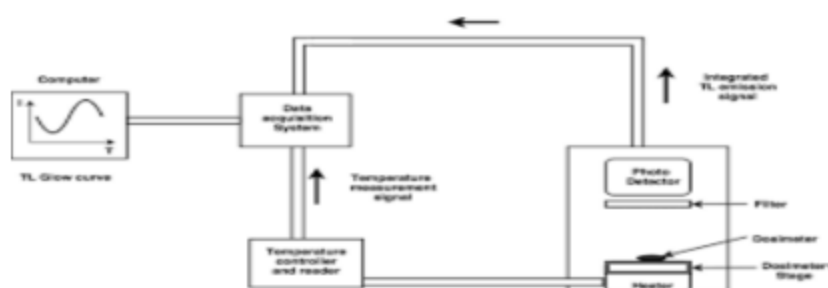
Fig. 2: A Schematic for TLD reader
