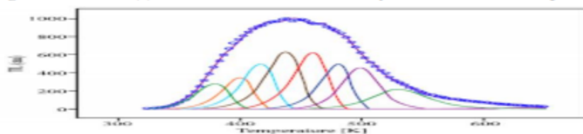
Fig. 3: Glow curve (b) fitting different peaks to wide curve
